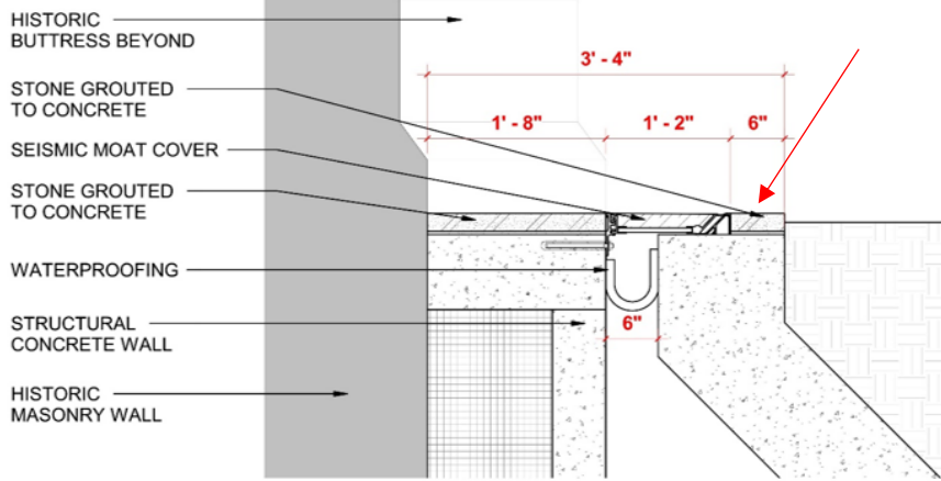
SEISMIC JOINT COVER WITH STONE EDGING
