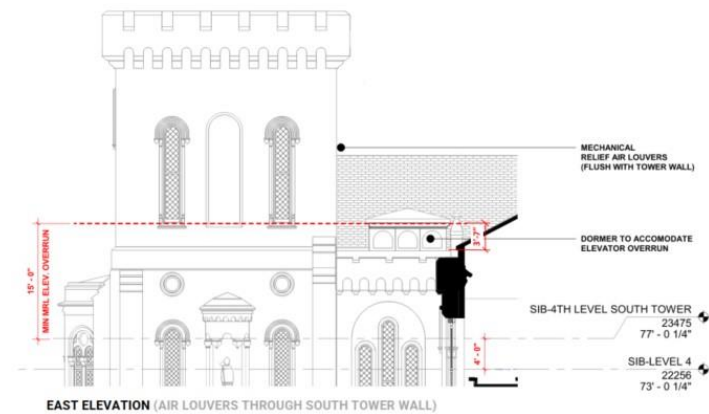
East elevation of the South Tower, depicting the preferred hipped roof and detailing of the overrun.
